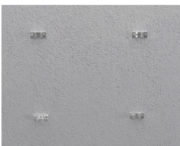
⑩. Using 11# Spare Parts (M8*60)
